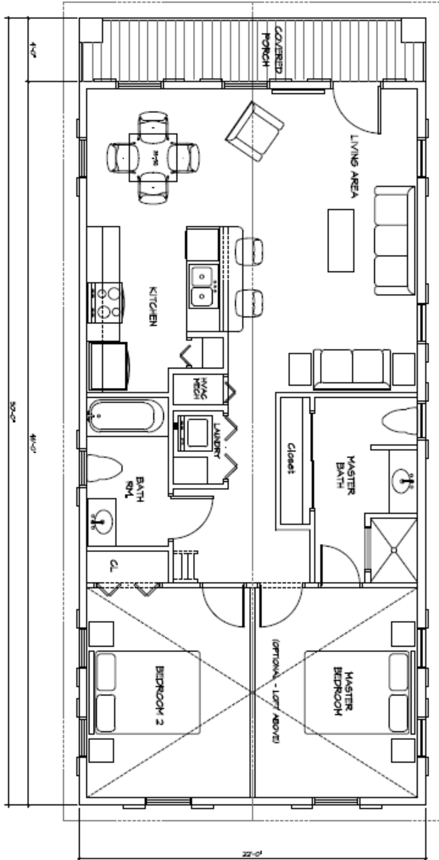
FLOOR PLAN
